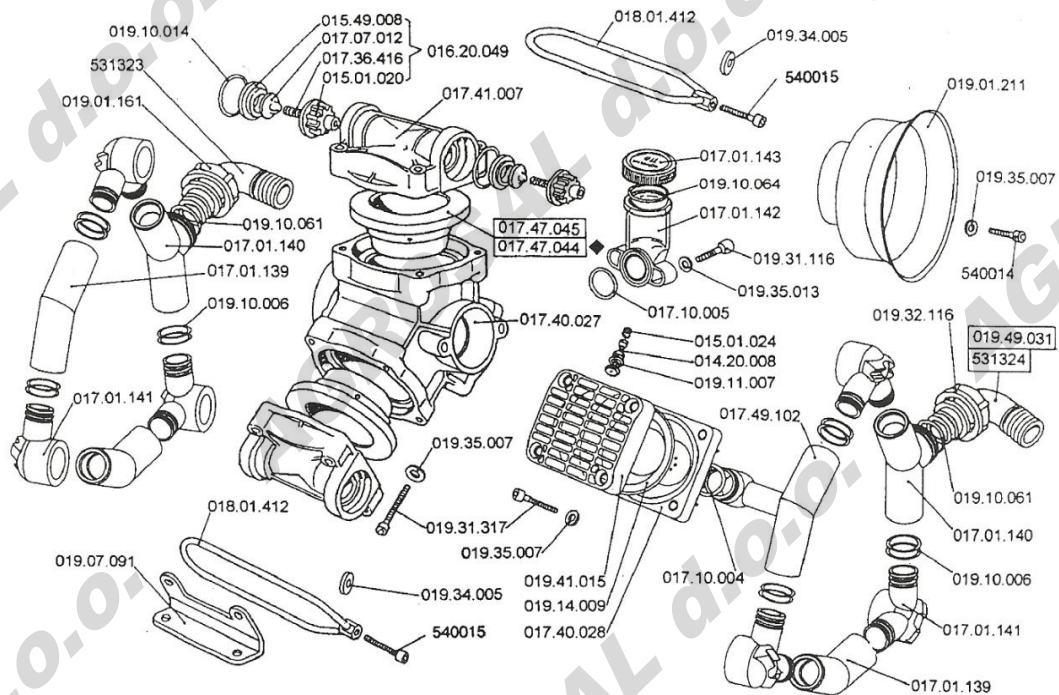
◆ BM120/20
