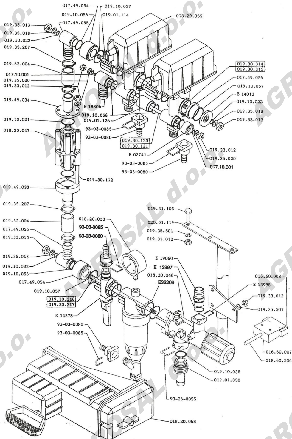
REGULATOR PR-3 EC
