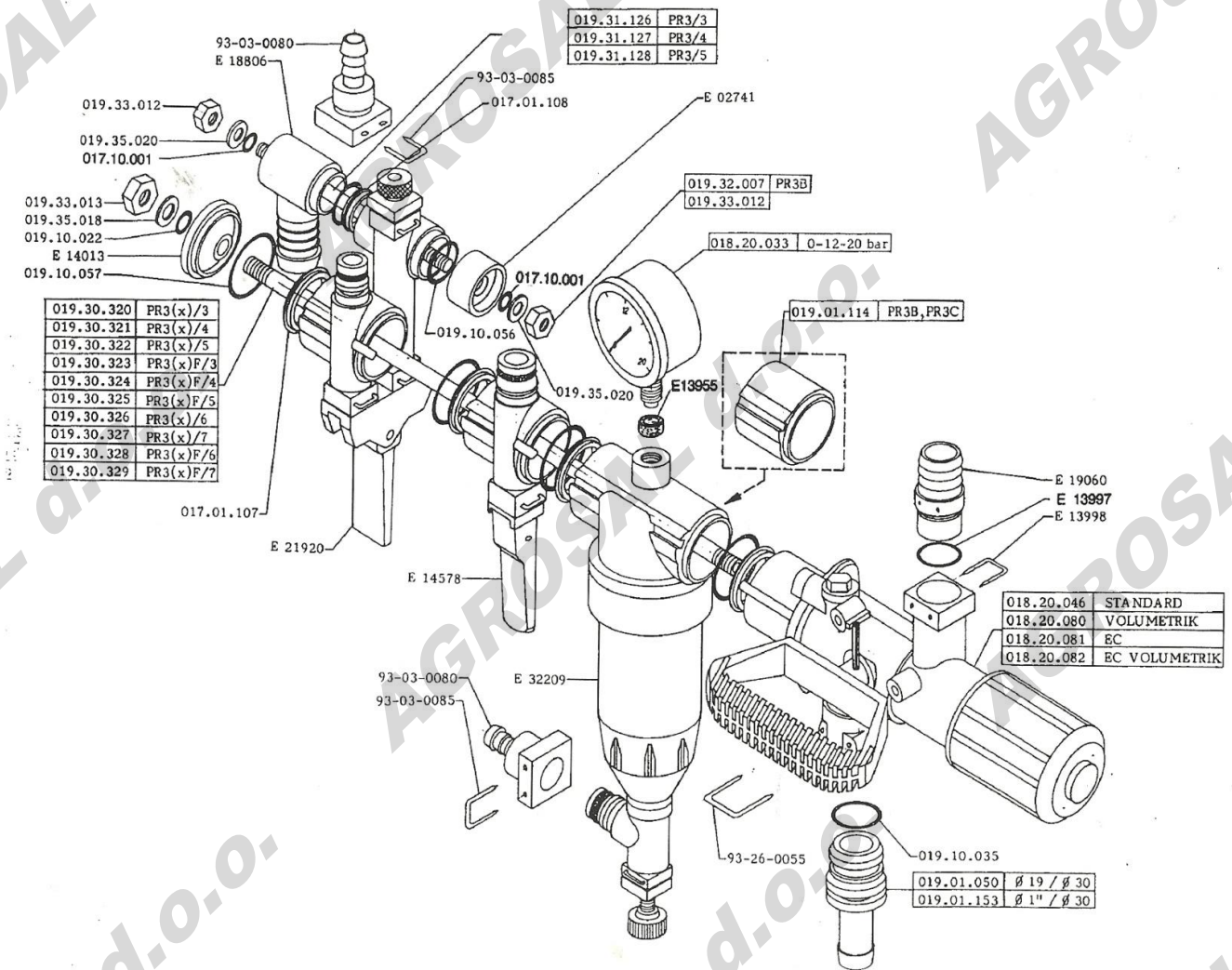
REGULATOR TLAKA PR-3
