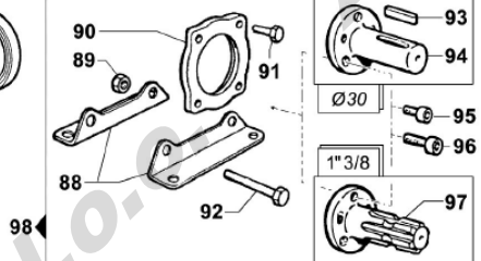
Kit / Optional Kit Cardano 1"3/8 - Kit Cardano Ø30 1"3/8 Cardan Kit - Ø30 Cardan Kit
