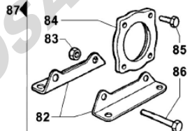
Kit / Optional Kit Piedi Pompa Feet Kit for Pump
