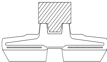
"RAIL TYPE" OUTER FLANGE TRACK ROLLER RULLO GUIDA ESTERNA ALTA
