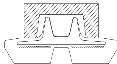
OUTER FLANGE TRACK ROLLER RULLO GUIDA
